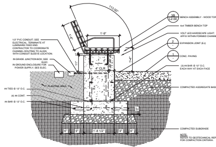
CONCRETE BENCH WITH WOOD TOP
